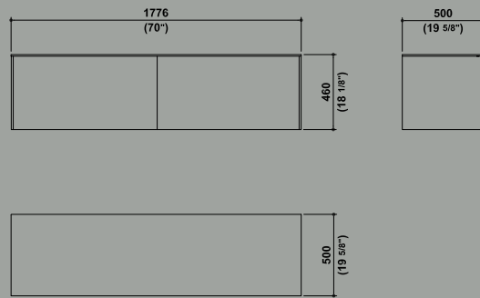
Morphing/unit mobile sospeso con doppio cassettone wall-mounted base unit with 2 pull-out drawers
