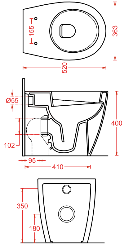
STV002 STEP vaso terra filomuro back to wall WC
